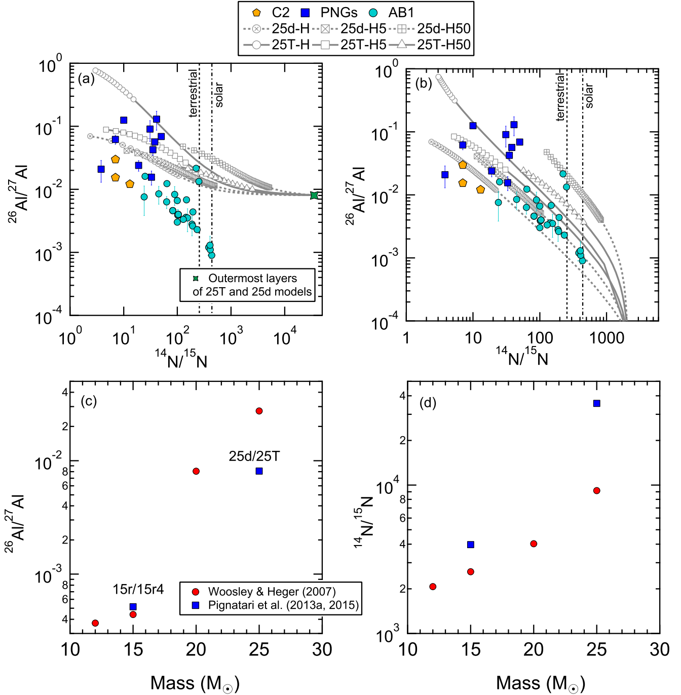
Figure 4. Upper panel: the same set of grain data in Figure 3 are compared to the predicted compositions of SN ejecta for N and Al isotope ratios. The model predictions are shown as mixing lines (lines with symbols represent C > O and lines represent C < O ) between pure explosive H-burning ejecta and (a) materials from the corresponding outermost layers in the 25d and 25T models, (b) the H-envelope material in the 12 M_{\odot} WH07 SN model. Bottom panel: plots of model predictions for ^{26}\text{Al}/^{27}\text{Al} and ^{14}\text{N}/^{15}\text{N} ratios in the outermost layers vs. the initial stellar mass of an SN.
