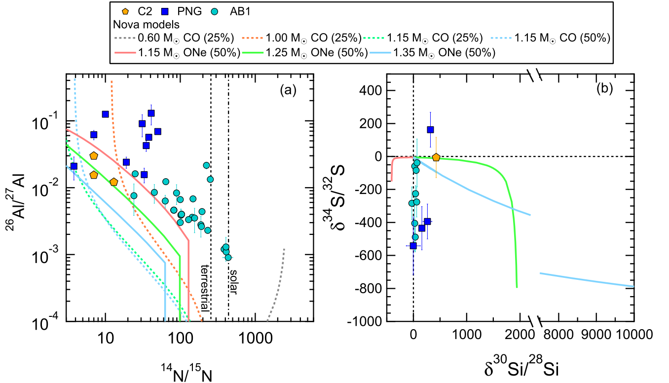
Figure 3. Plots of ^{26}\text{Al}/^{27}\text{Al} vs. ^{14}\text{N}/^{15}\text{N} and \delta^{34}\text{S}/^{32}\text{S} vs. \delta^{30}\text{Si}/^{28}\text{Si} for presolar SiC grains and nova models. AB grains and PNGs from this study and L16a are compared to the predicted compositions of CO and ONe nova ejecta (José & Hernanz 2007). The model predictions are shown as mixing lines between pure bulk nova ejecta and material of solar composition. For each nova model, the number in parentheses refers to the percentage of H-rich material accreted onto the white dwarf. The CO nova models predict quite close-to-solar Si and S isotope ratios and therefore cannot be seen in (b).
