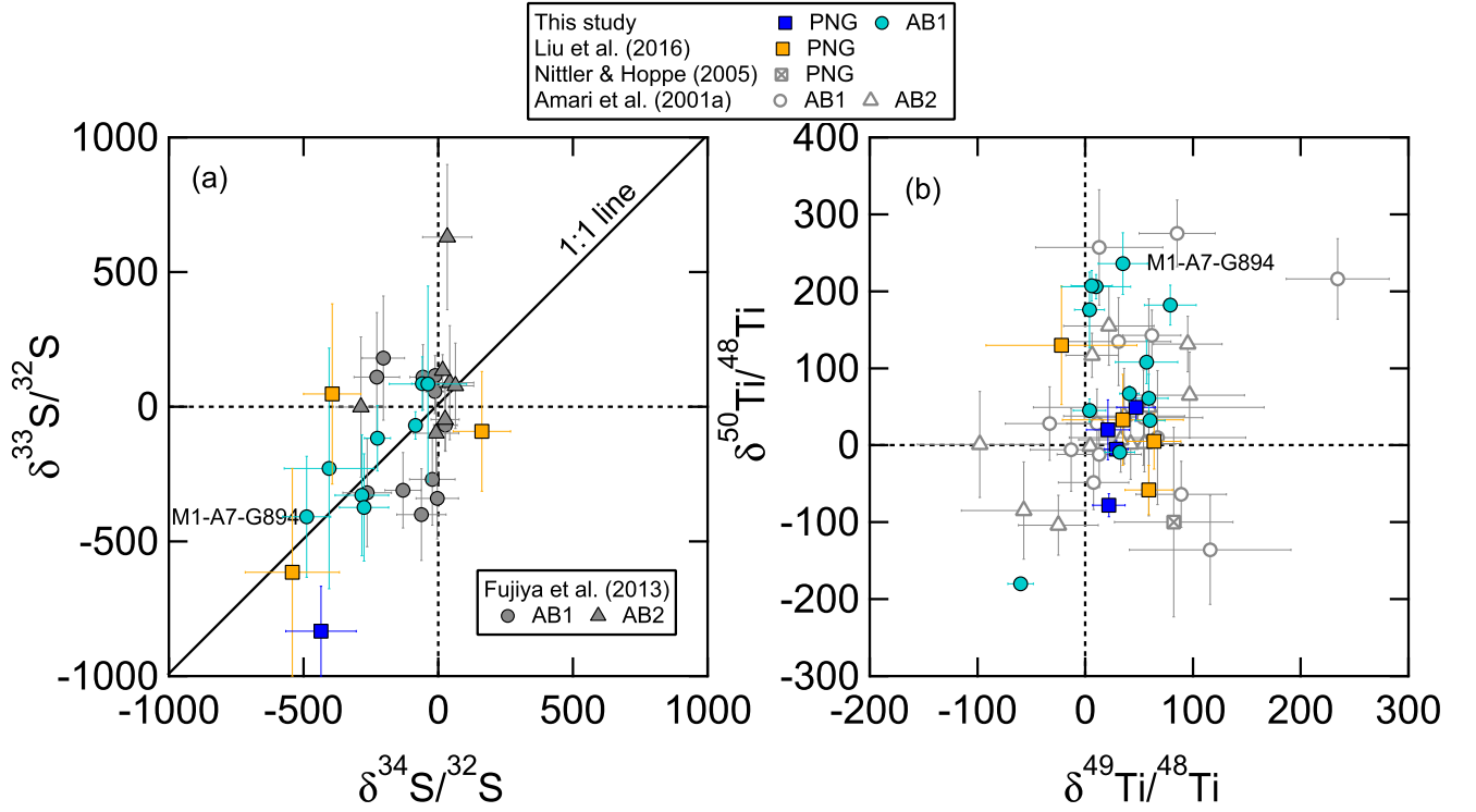
Figure 2. Isotopic compositions of S and Ti of SiC AB grains and PNGs from this study are compared to literature data.
