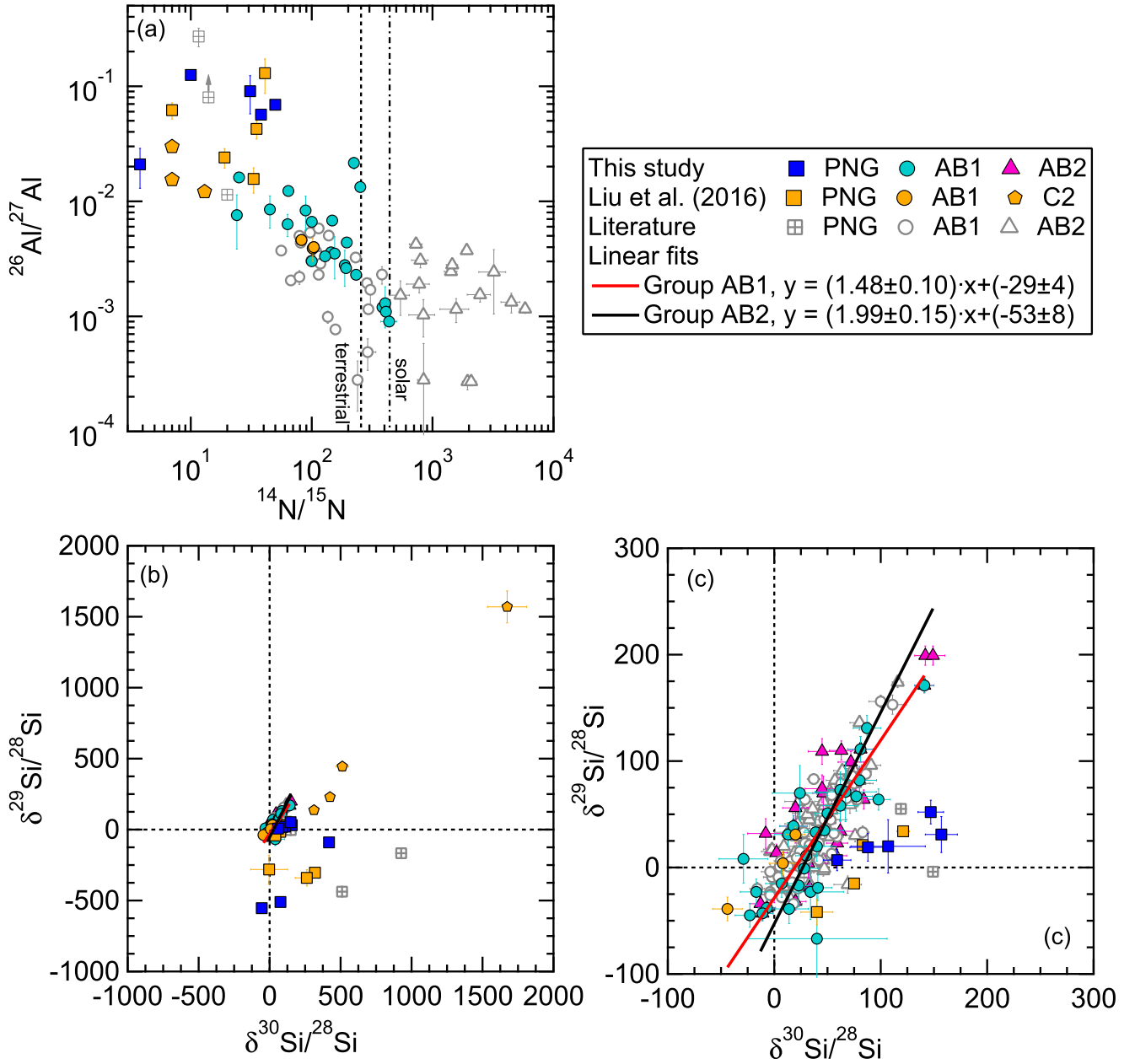
Figure 1. Isotopic compositions of N, Al, and Si of SiC AB grains and PNGs from this study are compared to literature data (Amari et al. 2001a, 2001b; Nittler & Hoppe 2005; L16a). For ^{14}\text{N}/^{15}\text{N} , the protosolar value of 441 \pm 5 reported by Marty et al. (2011) is shown as a dashed-dotted line for reference. The dashed lines represent terrestrial isotopic compositions. AB grains from this study and A01b were used for the linear fits. \delta^i\text{Si} is defined as [(^{i}\text{Si}/^{28}\text{Si})_{\text{grain}} / (^{i}\text{Si}/^{28}\text{Si})_{\text{std}} - 1] \times 1000 , where ^i\text{Si} denotes ^{29}\text{Si} or ^{30}\text{Si} , and (^{i}\text{Si}/^{28}\text{Si})_{\text{grain}} and (^{i}\text{Si}/^{28}\text{Si})_{\text{std}} represent the corresponding isotope ratios measured in a grain and the SiC standard, respectively.
